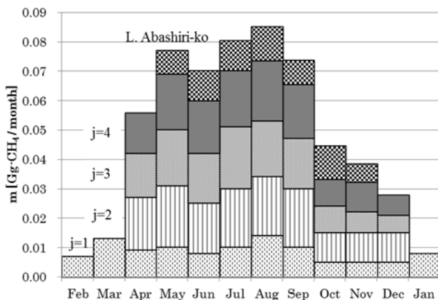
Fig. 9. Seasonal changes in mass flux from lakes in Hokkaido.
